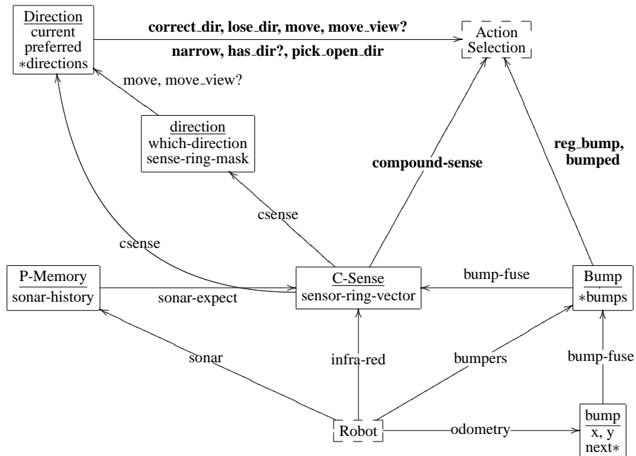
Fig. 2. The behaviors involved in moving a robot forward.
