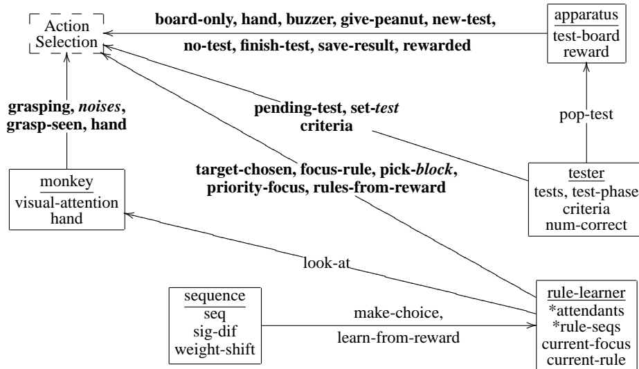
Fig. 4. Behaviors used for an artificial life model of transitive inference learning. Notice that this single BOD agent represents two real-world agents, a monkey and a testing apparatus.
