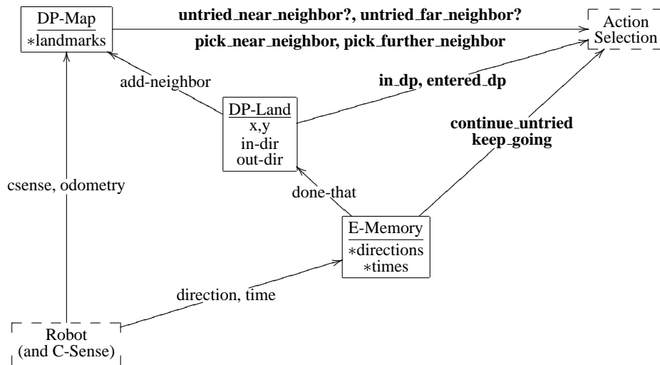
Fig. 3. Additional behaviors for map learning.
