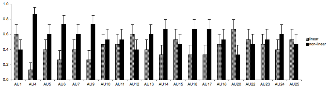
(a) Onset motion linear/nonlinear preference frequency for each AU (normalized)
