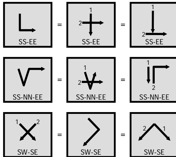
Figure 1. The recognition algorithm allows a signature to be accessed via different strokes.
