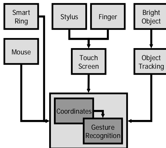
Figure 2. Using various techniques with the stroke recognition engine.
