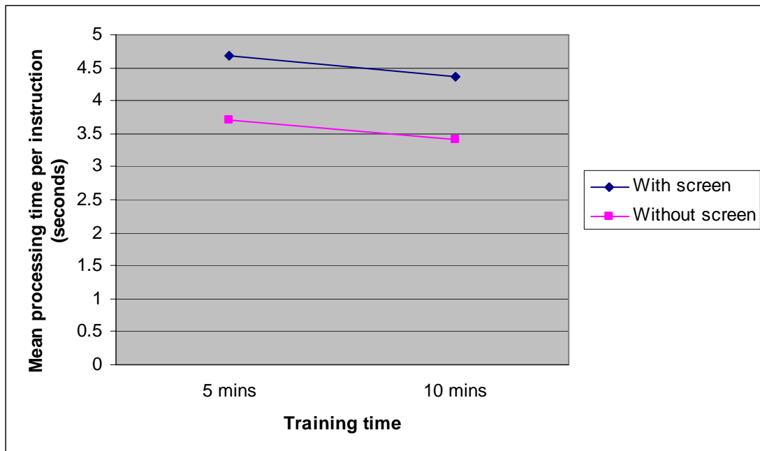
Figure 8. Interaction of factors on instruction processing time.
